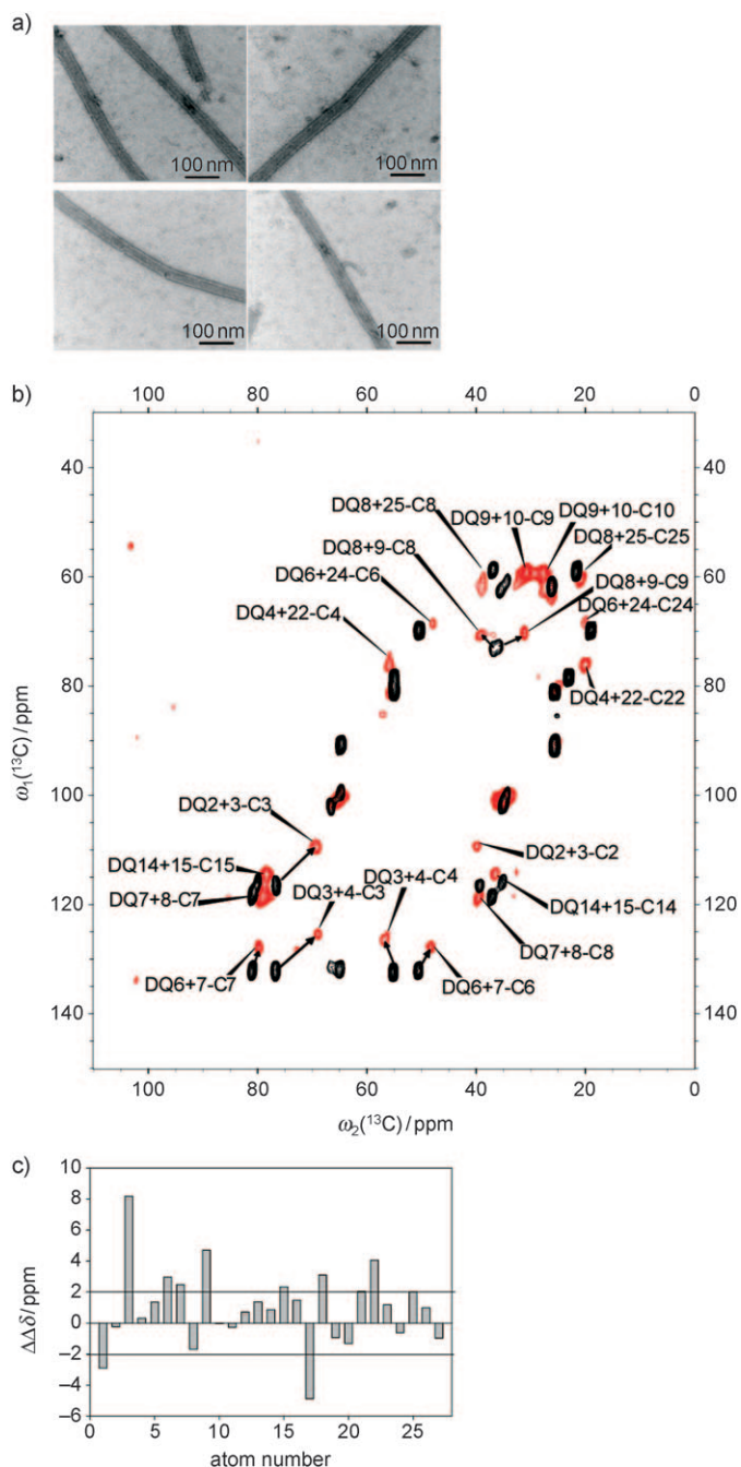
Figure 1. a) TEM image of microtubules complexed with patupilone. b) Aliphatic region of 2D ^{13}\text{C} – ^{13}\text{C} (2Q,1Q) NMR correlation spectra for free patupilone (black) and patupilone in a complex with MT (red). Cross-correlations for different atoms and strong signal shifts are indicated. c) Chemical-shift deviation of each carbon atom in patupilone upon binding to MT. The horizontal lines indicate approximately four times the (one-quantum) ^{13}\text{C} line width. This value is relevant for evaluation of the significance of chemical-shift differences.
